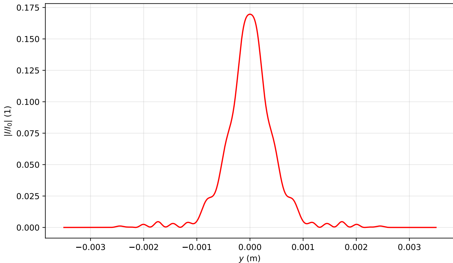
Intensity profile I(x=0, y, z=2.548)/I_0 , \text{Pin}=5.0\text{Pcr} , artificial time
